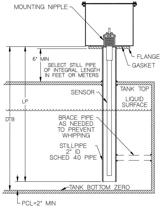
Figure 2.1 Stillpipe Mounting
