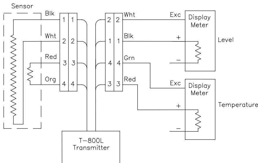
Figure 2.7 Level/temperature wiring to display with excitation
