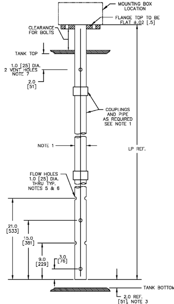
CONSTRUCTION DETAIL
