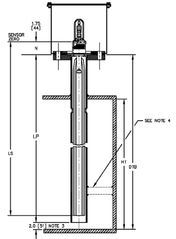
LENGTH DETAIL
