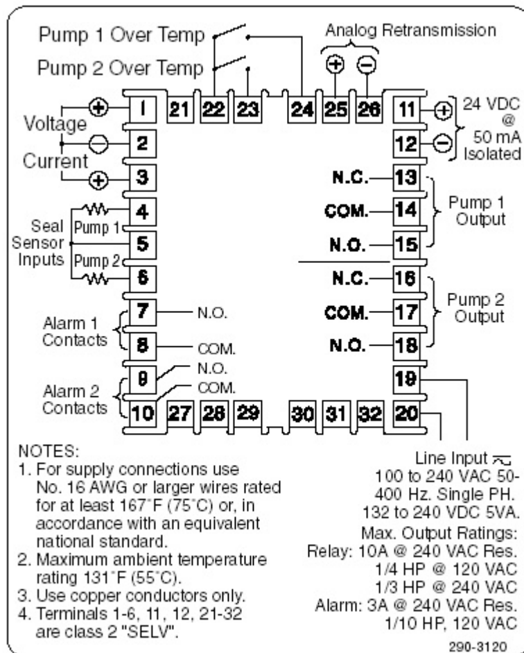
Figure 2 - Wiring
