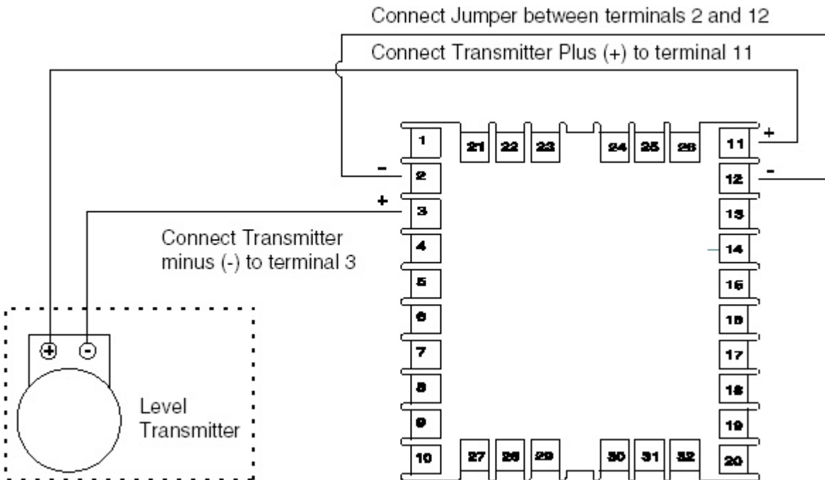
Figure 3 - Transmitter Wiring
