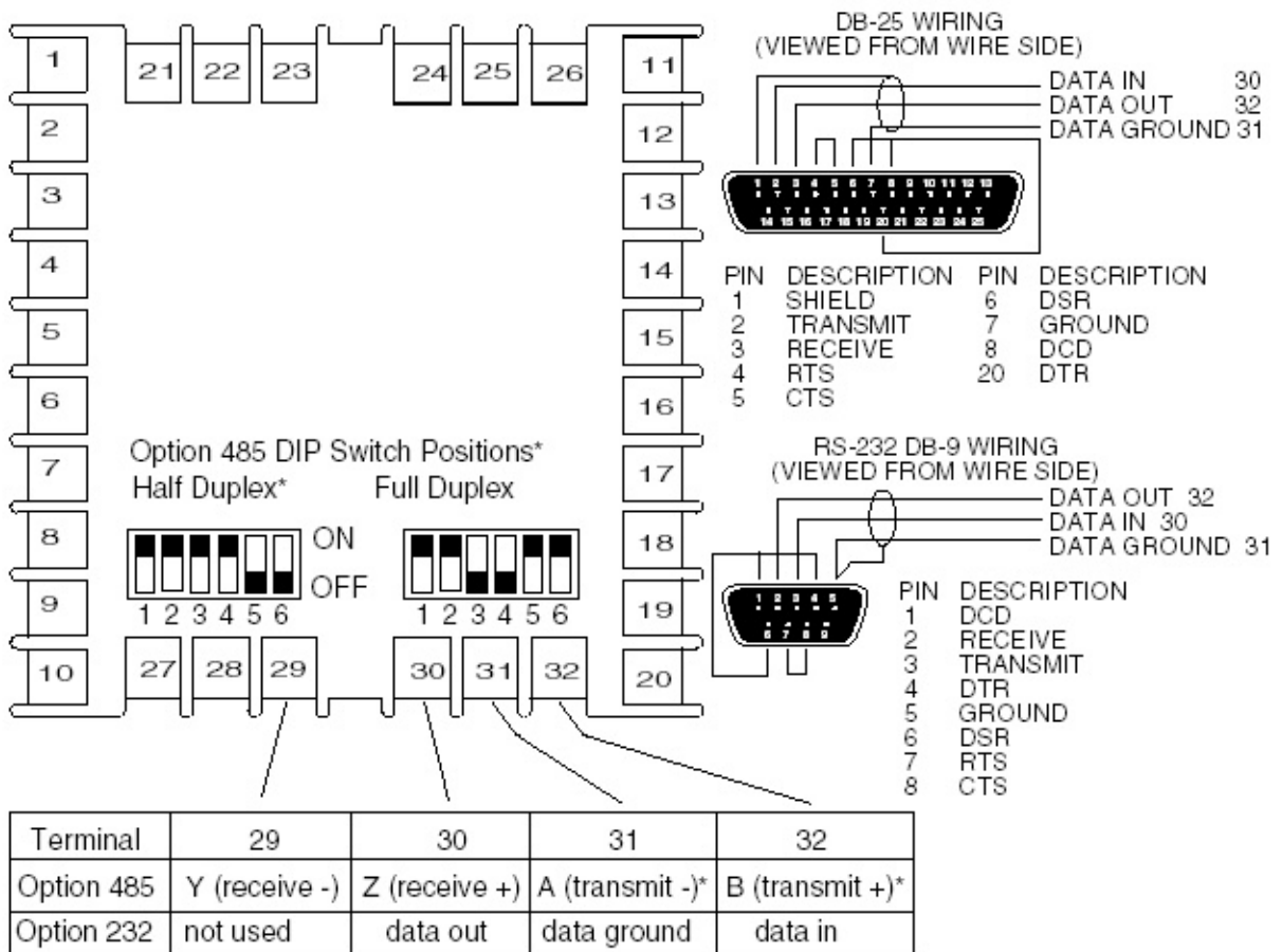
Figure 4 – Wiring for Options
